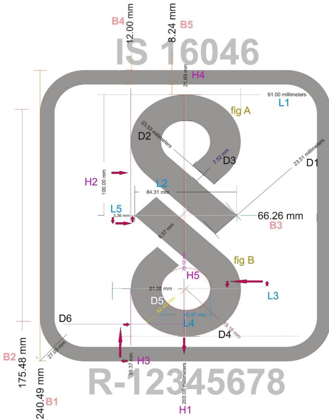
All dimensions in Millimeters
